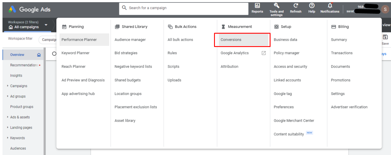
[Screenshot 1.1]
