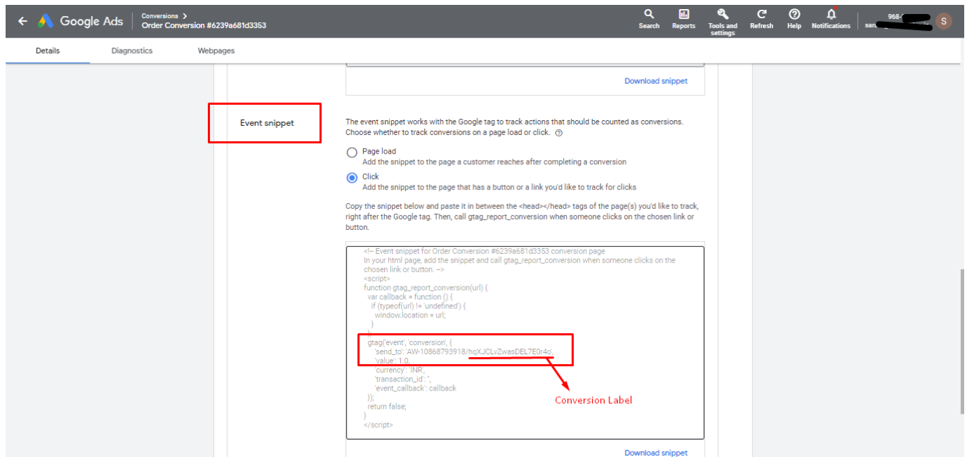
[Screenshot 5.1]
